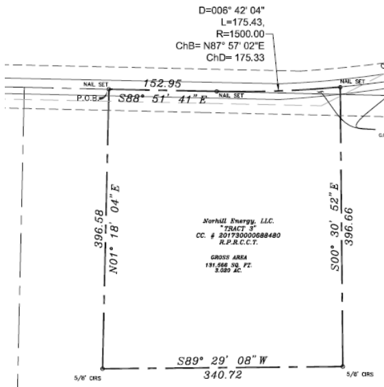
Southeast Corner
