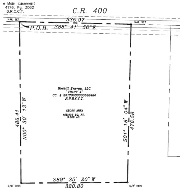
Southwest Corner
